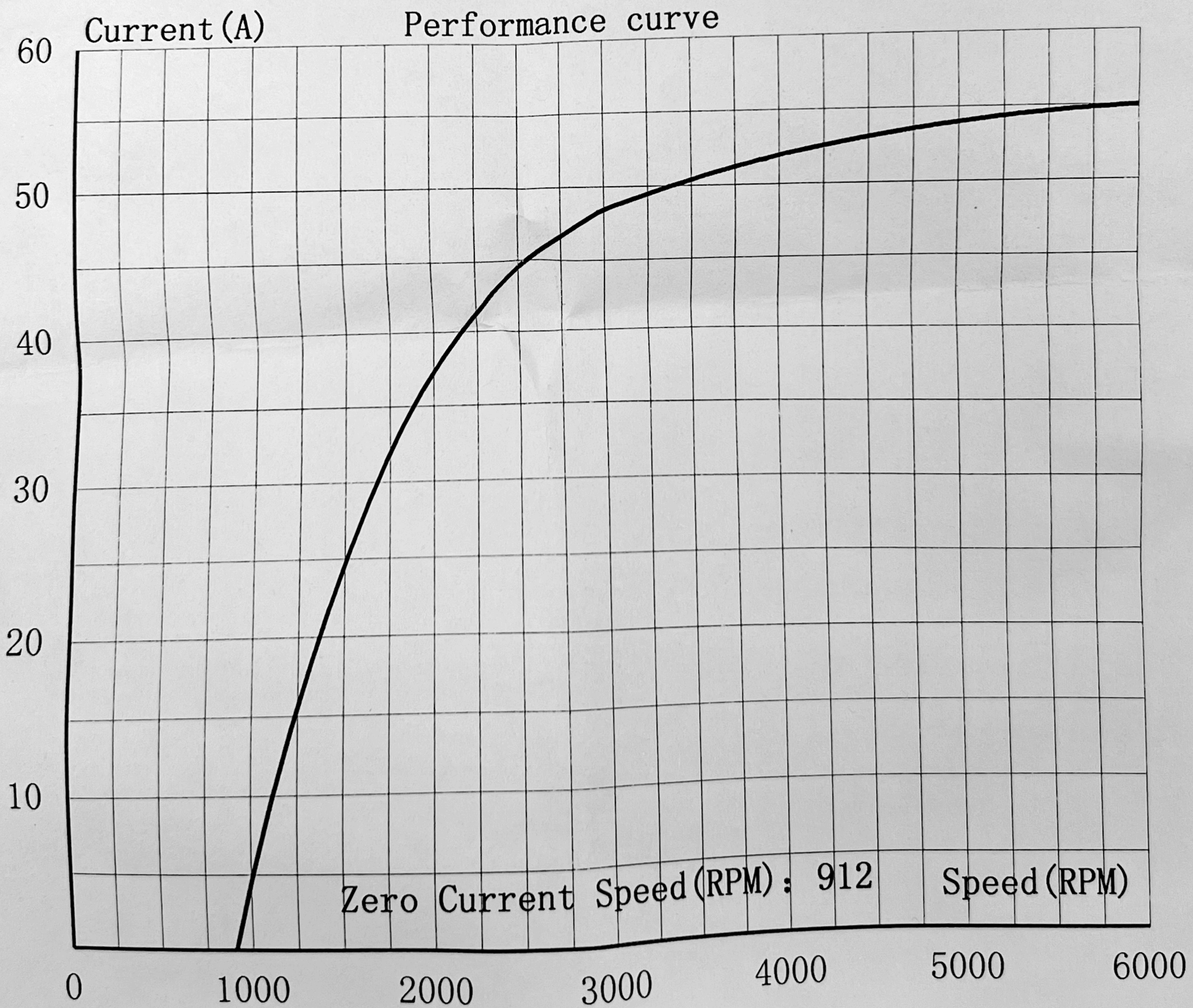
Speed Vs Current Table
